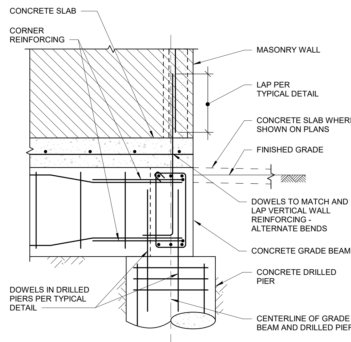
106 MASONRY WALL END OR CORNER AT CONCRETE GRADE BEAM AND DRILLED PIER S-401 NOT TO SCALE 17-036
