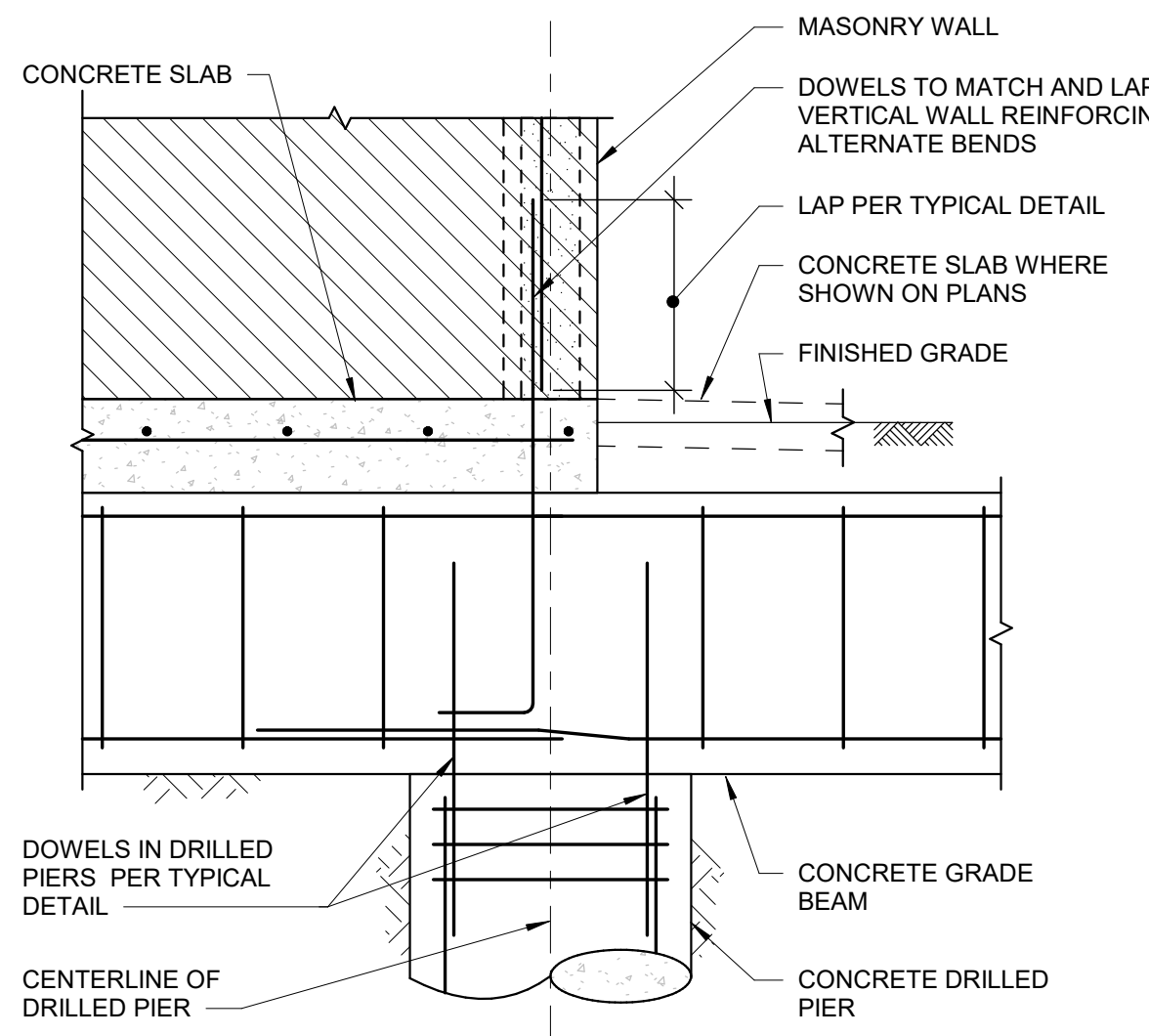
107 MASONRY WALL END OR CORNER AT CONCRETE GRADE BEAM AND DRILLED PIER S-401 NOT TO SCALE 17-036
