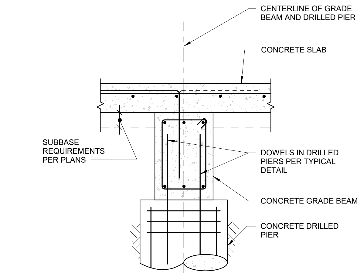
110 GRADE BEAM AT CONCRETE DRILLED PIER S-401 NOT TO SCALE 17-036
