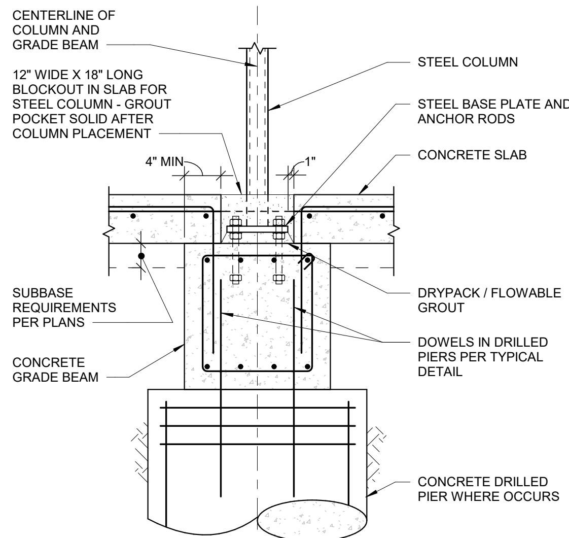
108 INTERIOR STEEL COLUMN FOOTING S-401 NOT TO SCALE 17-036
