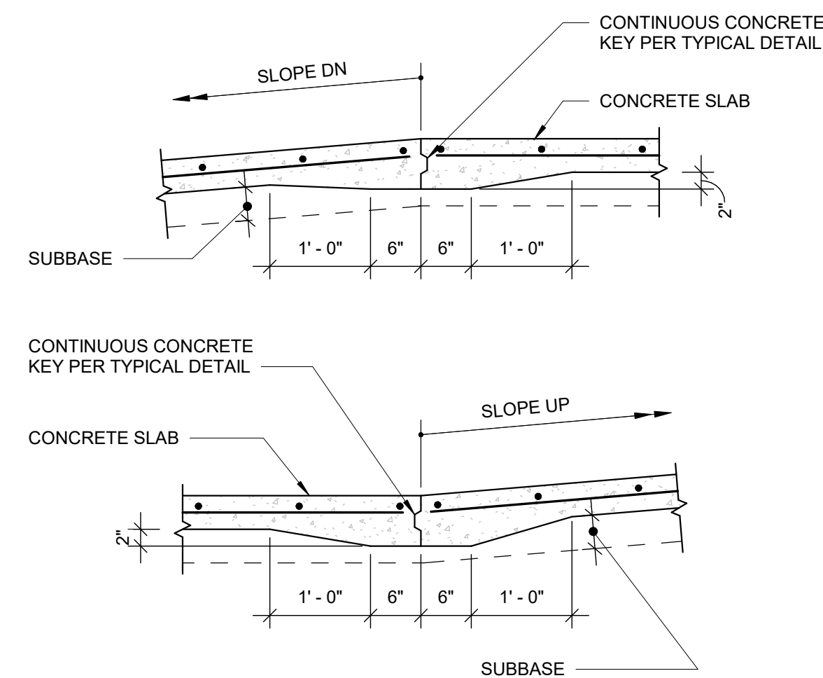
112 CONSTRUCTION JOINT IN CONCRETE RAMP S-401 NOT TO SCALE 17-036
