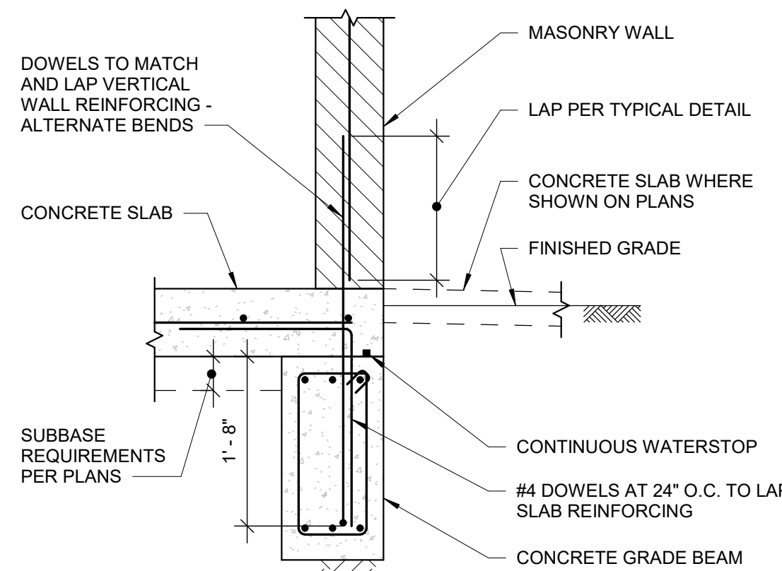
104 EXTERIOR MASONRY WALL AT GRADE BEAM S-401 NOT TO SCALE 17-036
