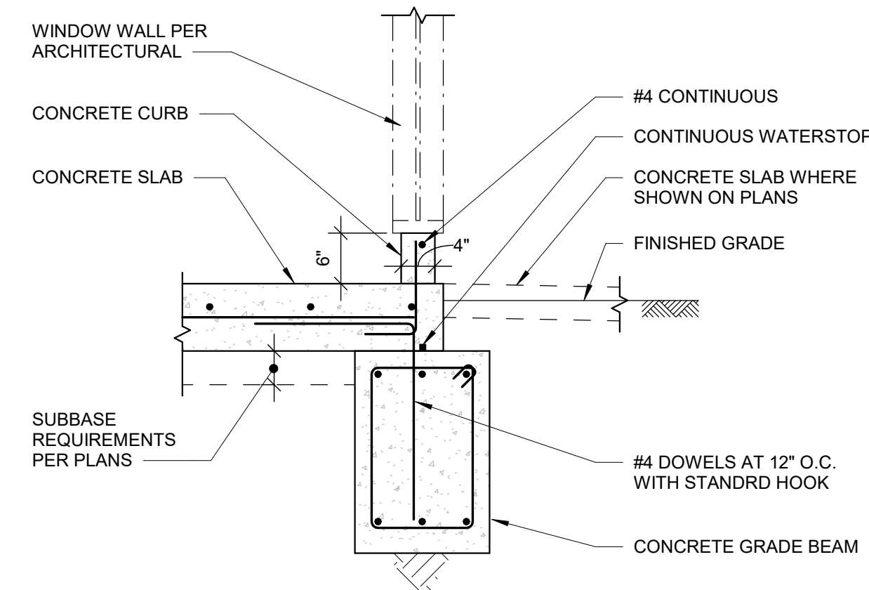
111 CONCRETE CURB AT WINDOW WALL S-401 NOT TO SCALE 17-036
