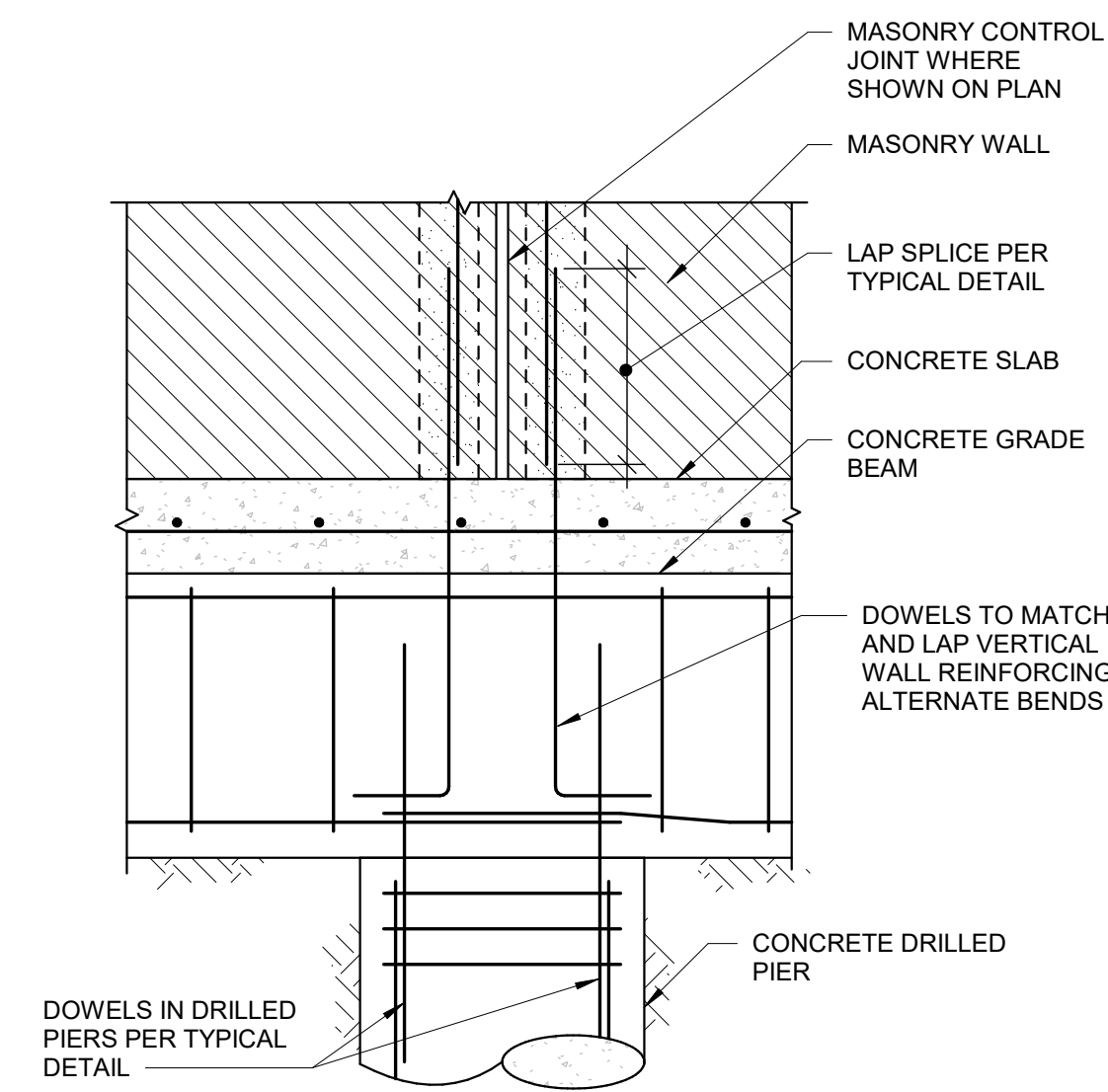
109 MASONRY WALL, CONCRETE GRADE BEAM AND DRILLED PIER AT MASONRY CONTROL JOINT S-401 NOT TO SCALE 17-036
