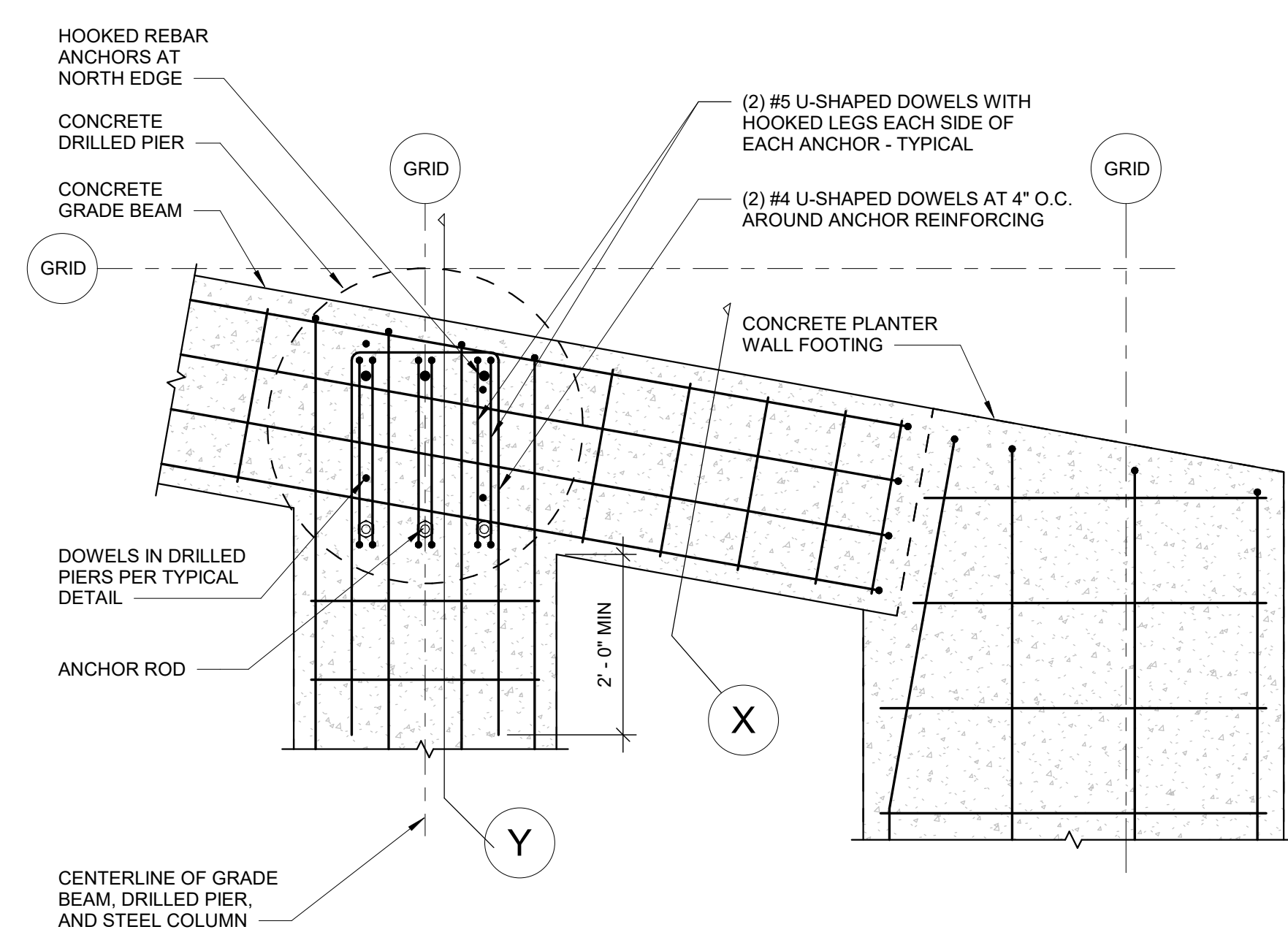
144 PLAN VIEW - STEEL COLUMN AT CONCRETE GRADE BEAM S-404 NOT TO SCALE 17-036
