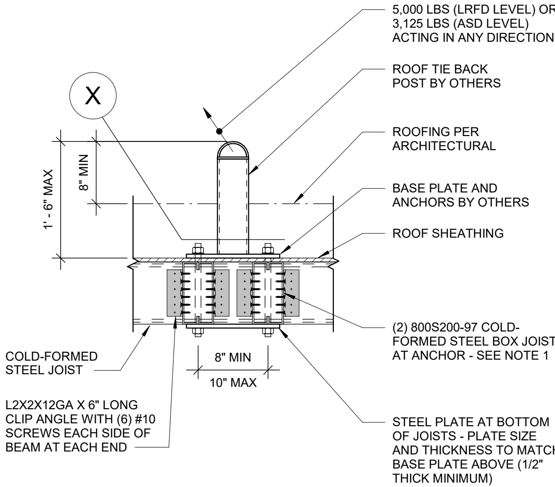
241 ROOF TIE BACK AT STEEL JOISTS S-504 NOT TO SCALE 17-036
